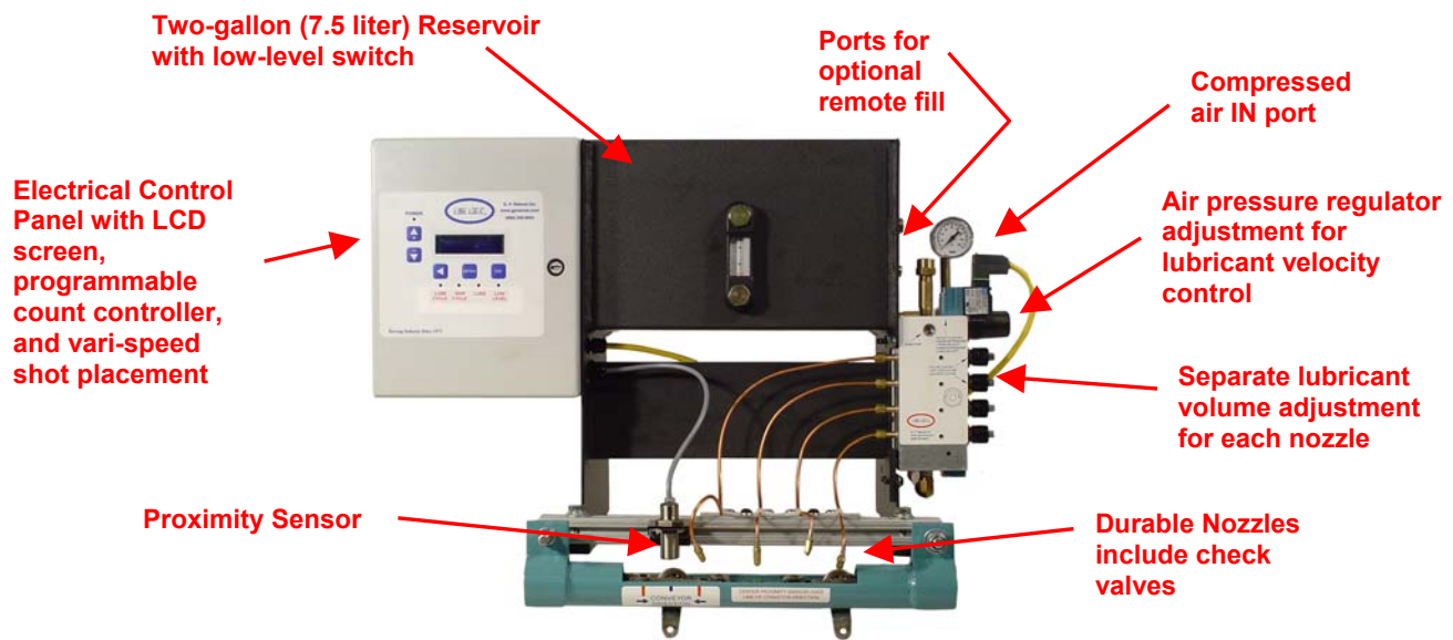
Photo shows SS6045 (for 200 series conveyor)
